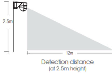
Wall-mount (Side)
