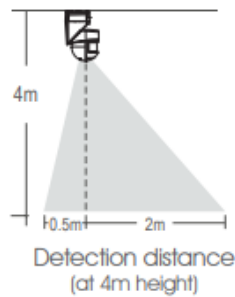
Ceiling-mount (Bottom)
