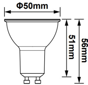
RE05/GU10 RE05DIM/GU10
