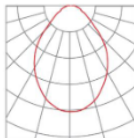
Microprism PS Diffuser 80°
