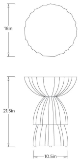
FAS18 NEREO CHISELED CONCRETE OUTDOOR ACCENT TABLE
