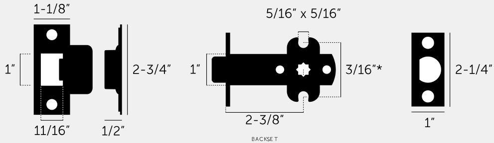
STRIKE PLATE
