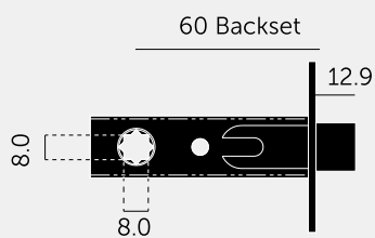
60MM, PASSAGE, 2 WAY
