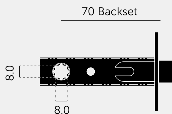
70MM, PASSAGE, 2 WAY
