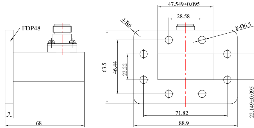
Dimensions are in mm
