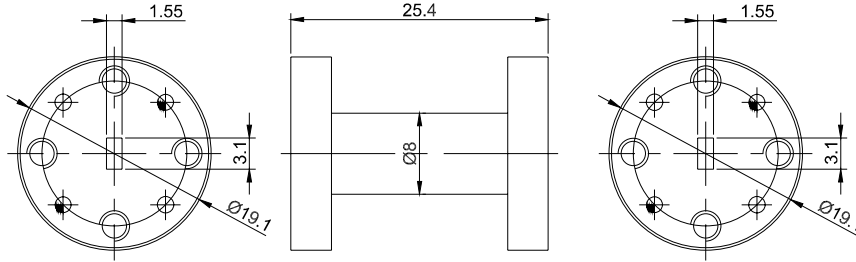
Dimensions are in mm
