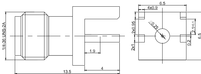
Dimensions are in mm
