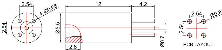
Dimensions are in mm
