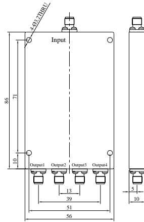
Dimensions are in mm
