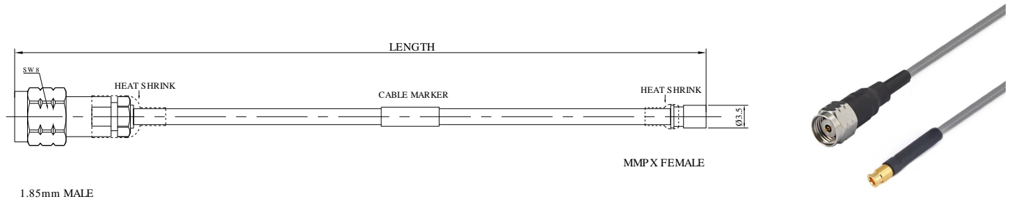
1.85mm MALE
