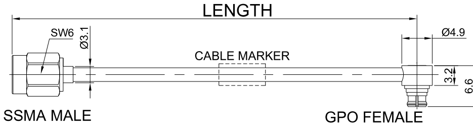
Dimensions are in mm
