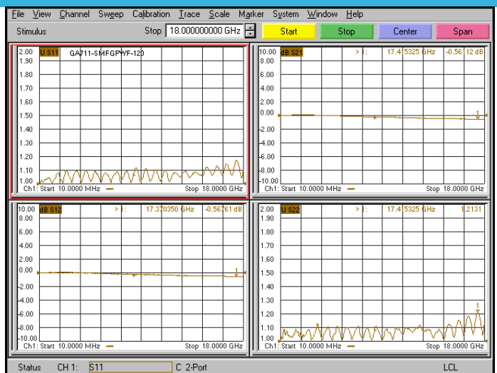
*Note: Test Cable Assembly Length = 120 mm
