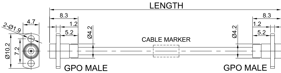
Dimensions are in mm
