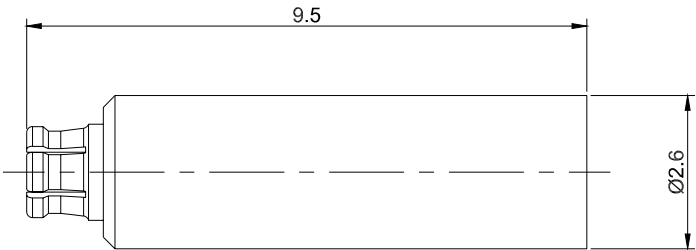
Dimensions are in mm
