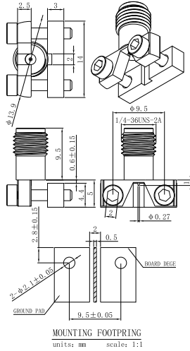
Dimensions are in mm
