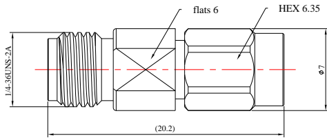
Dimensions are in mm
