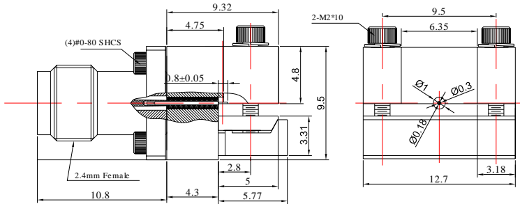
Dimensions are in mm
