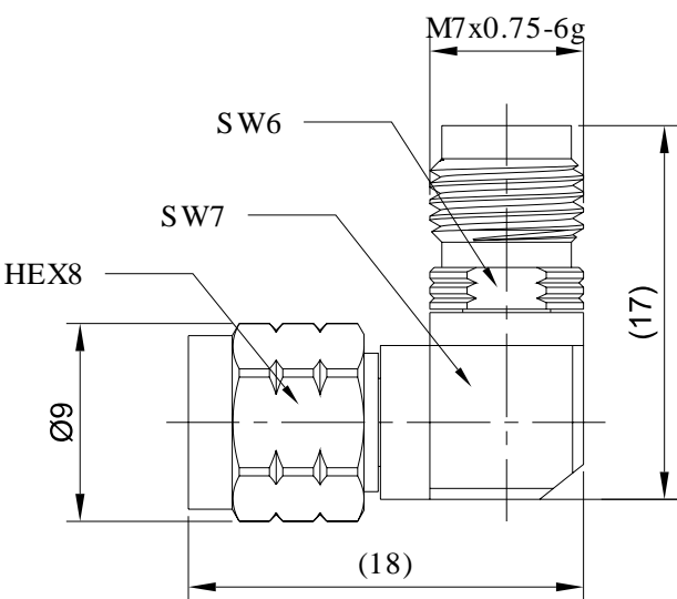
Dimensions are in mm
